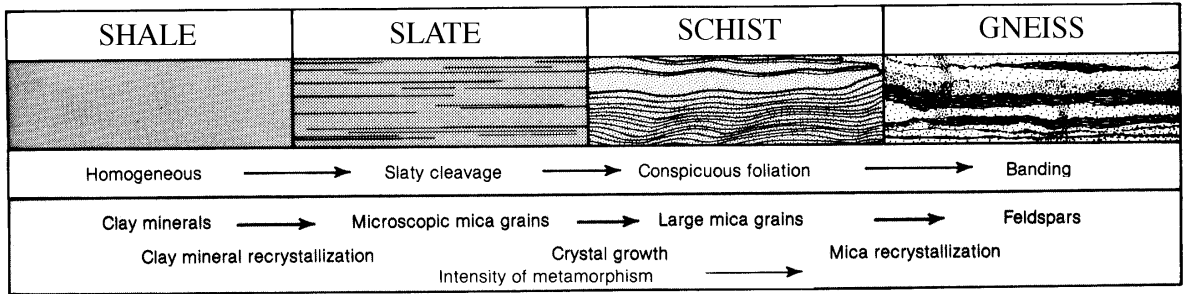
Figure 6-3. The textural changes associated with the metamorphism of a shale with increasing metamorphic grade.
